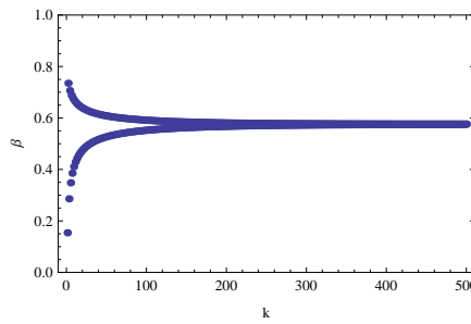
Figure 3: The ratio \beta for equation (14).
